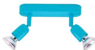
G12029/03 GU10, ES50 ▷ max. 2 × 50W ☑ 03, blue ☑ S20, metal ☒ 180mm ☒ 140mm CE ▽ ⊕ ✕ AC
