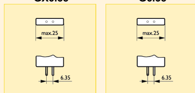
GX6.35
