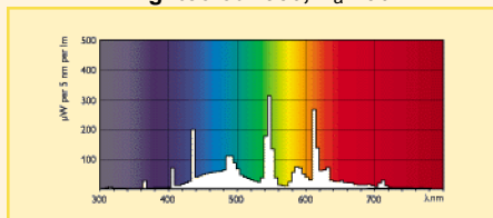
Lightcolour 950, R_a > 90
