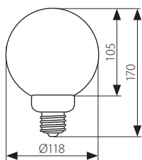
SUPERGLOB XEU38-20G
