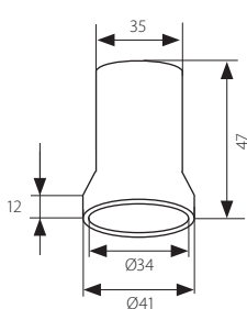
CP800D-E27
