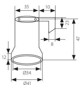
CP800F-E27
