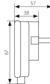
PIN W/US
