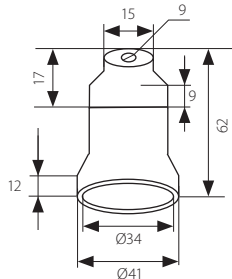
CP800D-E27
