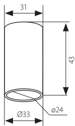
HLDR-E14
